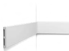
SX163 | SX163F SQUARE Duropolymer® 200 x 10,1 x 1,3 cm
