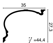
C344 HERITAGE Purotouch® 200 x 27,3 x 35 cm
